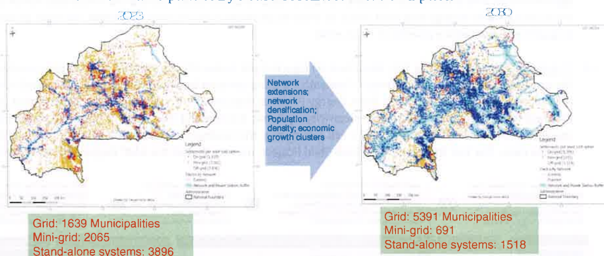
Figure 5: Maps showing municipalities with least cost electrification options in Burkina Faso
